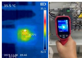
breaker Inverter No.1 35.5 °C
